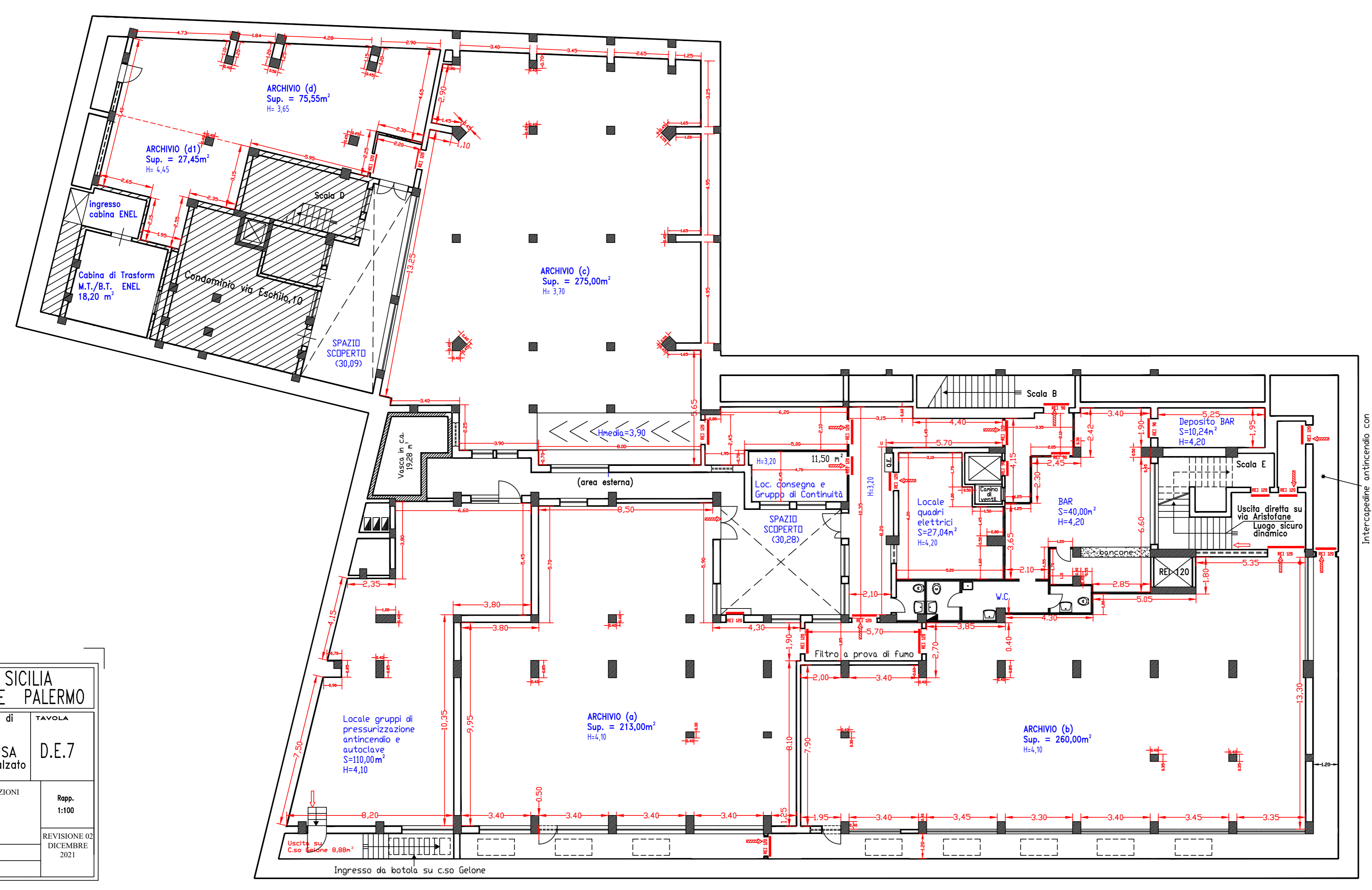
PIANO SEMINTERRATO
