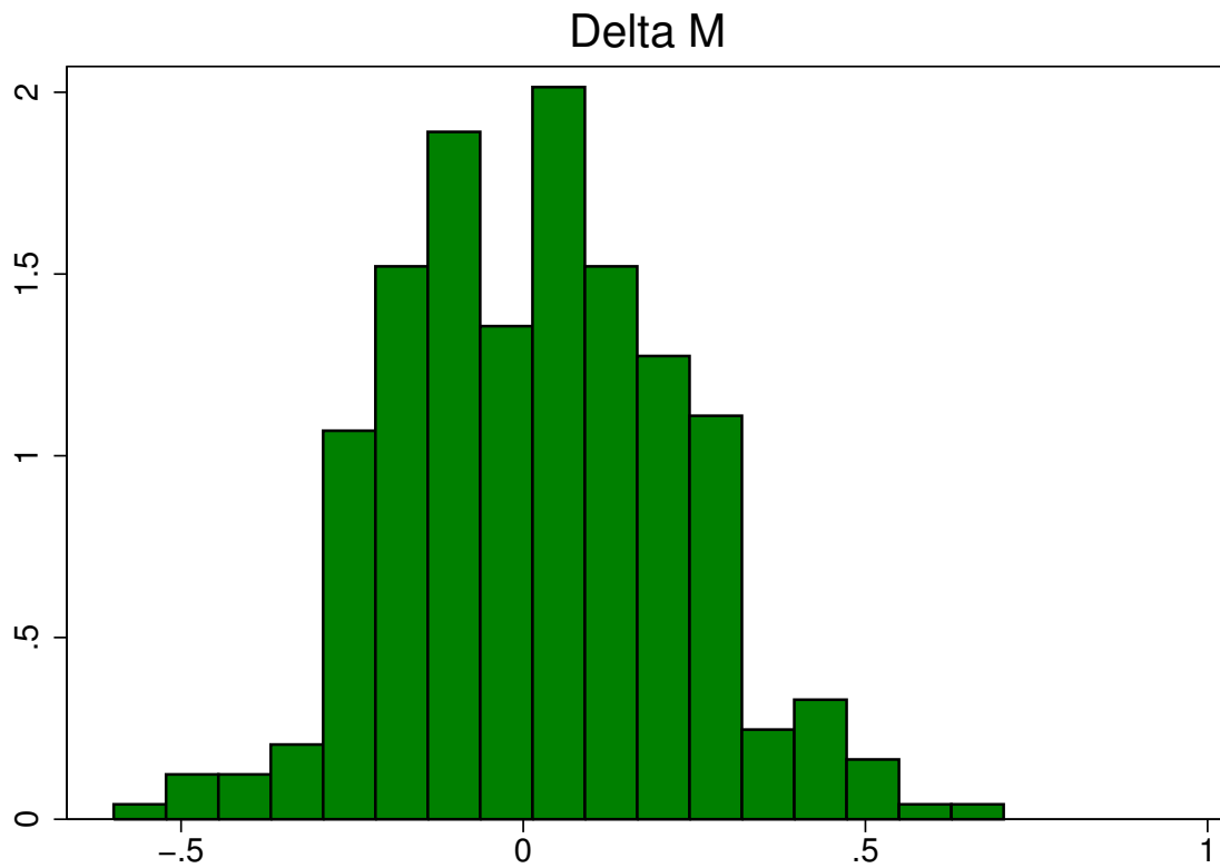
Figure J.V: Treatment Intensity for Events Balanced on [-4, 6]
